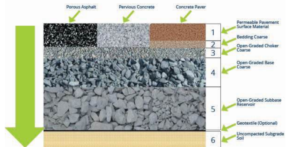
Figure 4.8: Illustration of typical layers in a previous pavement system, showing how porous surfaces and underground base materials allow rainwater to infiltrate and reduce runoff.
