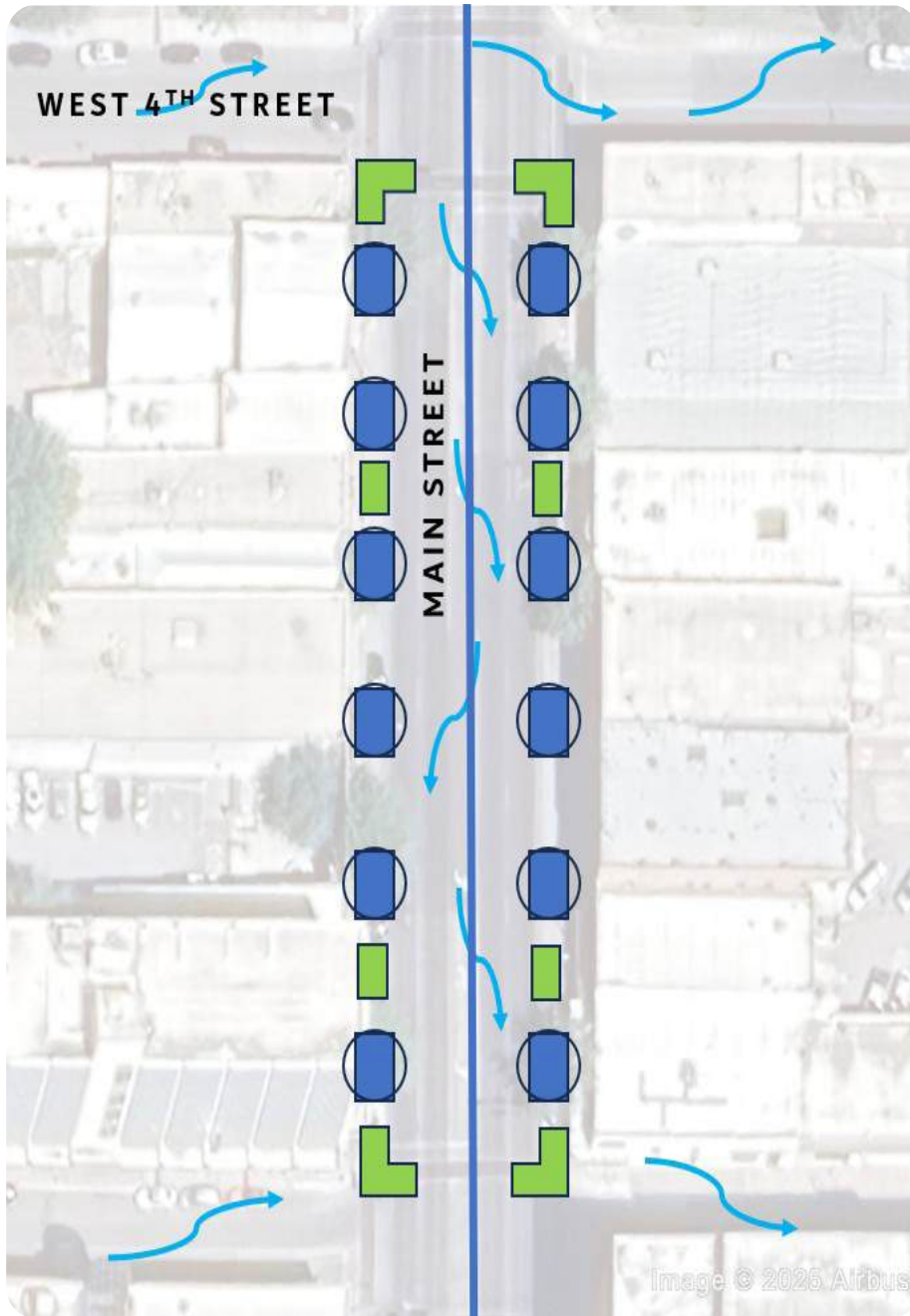
Figure 8.5 (A,B,C,D): Represents proposed water retention strategies for Main Street with the use of green infrastructure, including bio-retention planters, tree trenches, and depressed tree pits, to manage stormwater runoff. These tools capture and infiltrate rainwater from sidewalks and streets, helping reduce flooding, support tree health, and improve long-term water sustainability downtown.
