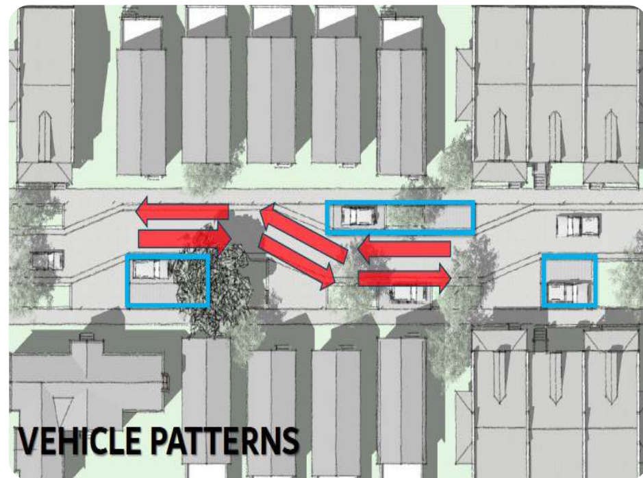
Figure 4.6 (A, B, C, D): Illustrate how W 7th Street can evolve from an underused corridor into a multi-functional public space: re-designing vehicle patterns, adding permeable green areas and integrated traffic calming measures transform the street into a safer, more flexible environment that supports stormwater management, pedestrian activity and community gathering.
